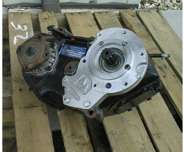
Side view of the transfer case and adapter.
