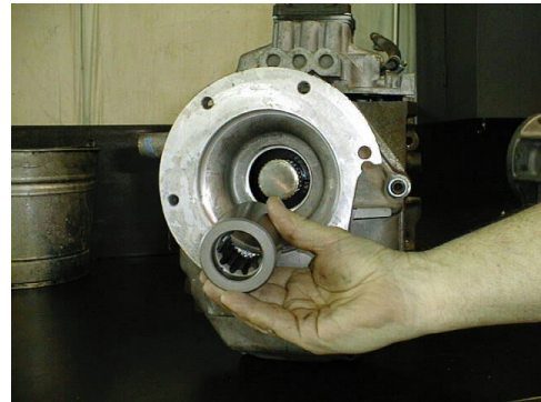
New coupler for 31 spline.
