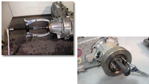
(Fig. 3) Slinger Removed / Harmonic Dampener
